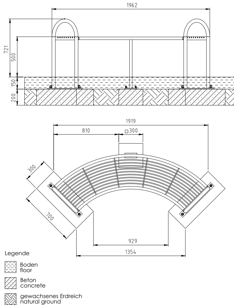
Diagram 2: Foundation plan
